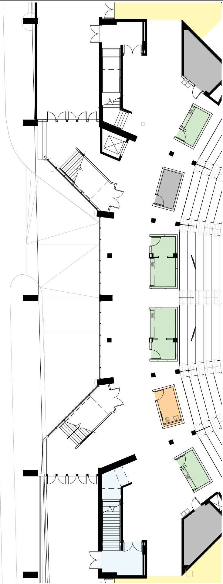
2 LEVEL 61 West - Existing Plan 2 1" = 20'-0"
