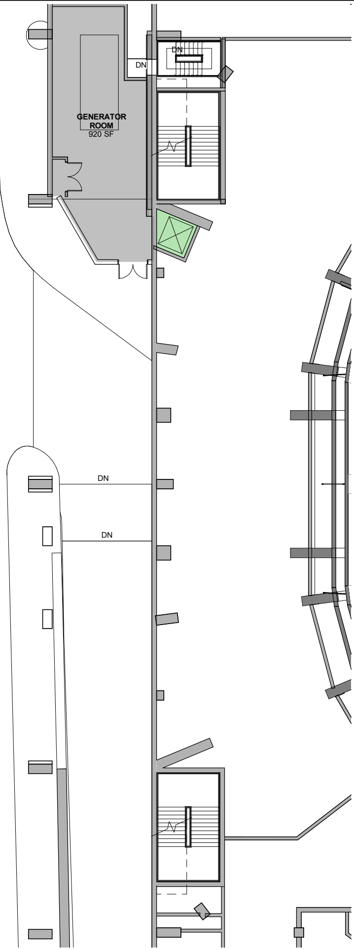
2 LEVEL 48 Sports Betting Plan 2 Opt 3 1" = 20'-0"
