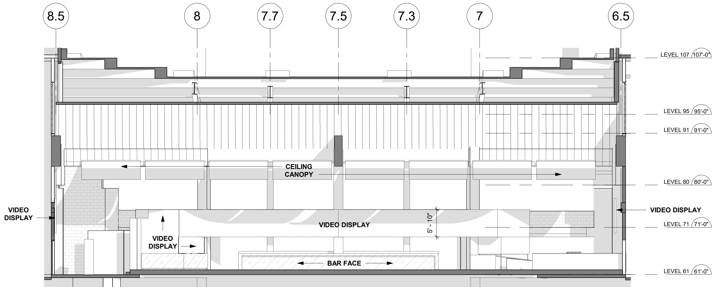
1 SPORTSBOOK BAR ELEVATION 3/32" = 1'-0"
