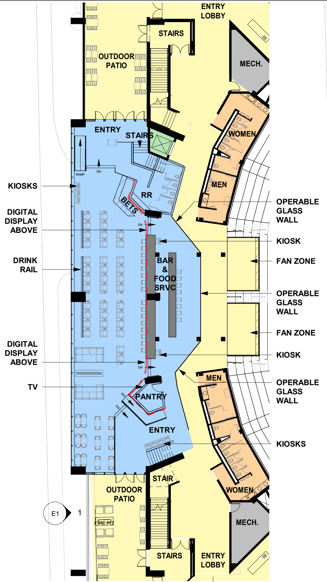
1 LEVEL 61 Sports Betting Plan 2 1" = 20'-0"
