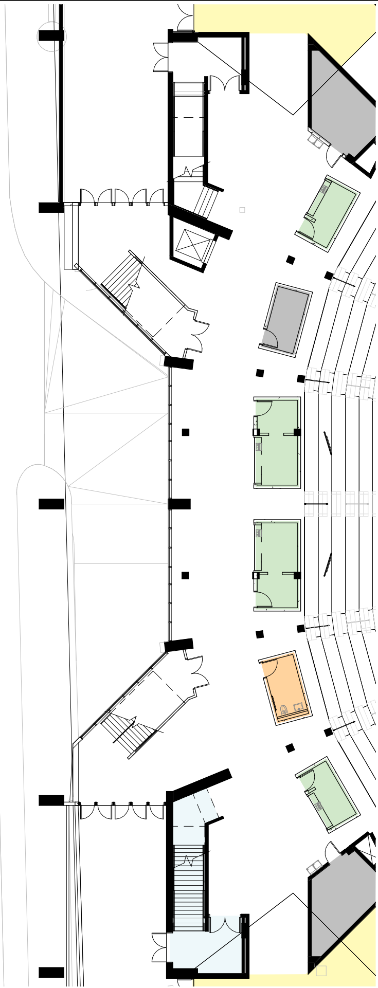
3 LEVEL 61 West - Existing Plan 2 Opt 3 1" = 20'-0"
