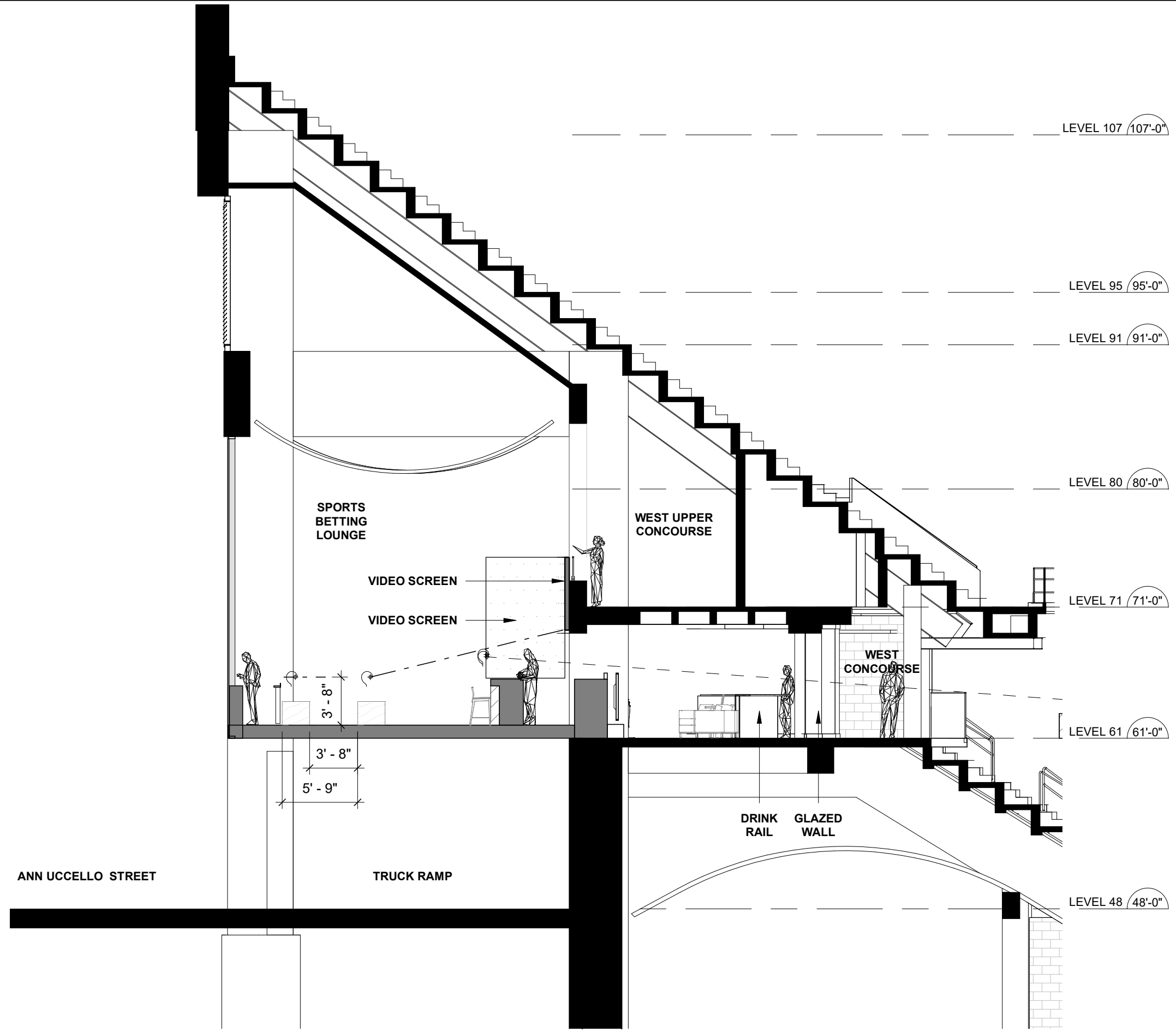
1 SPORTS BETTING - NORTH SECTION 1/8" = 1'-0"
