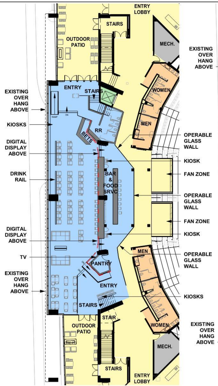
1 LEVEL 61 - SPORTS BETTING LOUNGE PLAN 1" = 20'-0"
