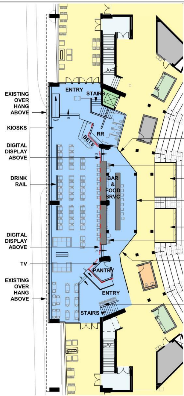
1 LEVEL 61 - SPORTS BETTING LOUNGE PLAN 1" = 20'-0"
