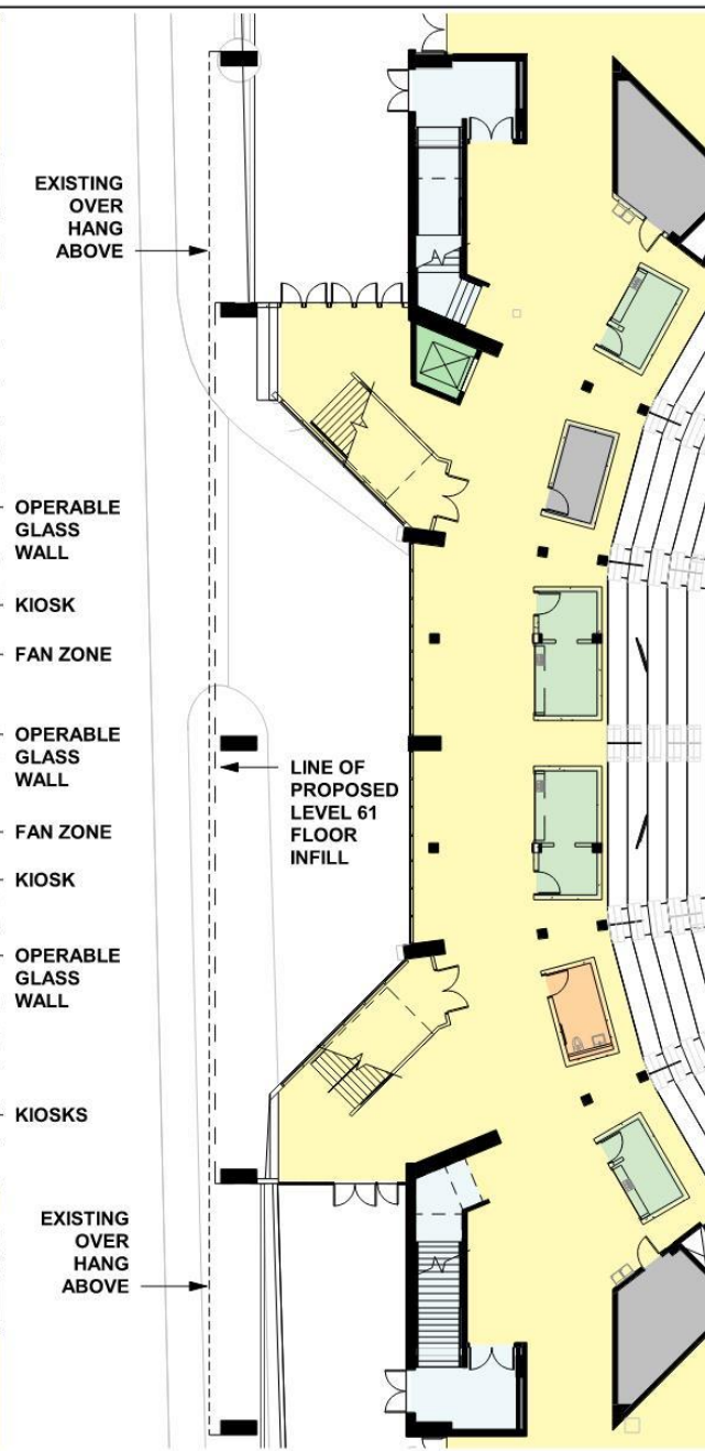
2 LEVEL 61 WEST - EXISTING FLOOR PLAN 1" = 20'-0"
