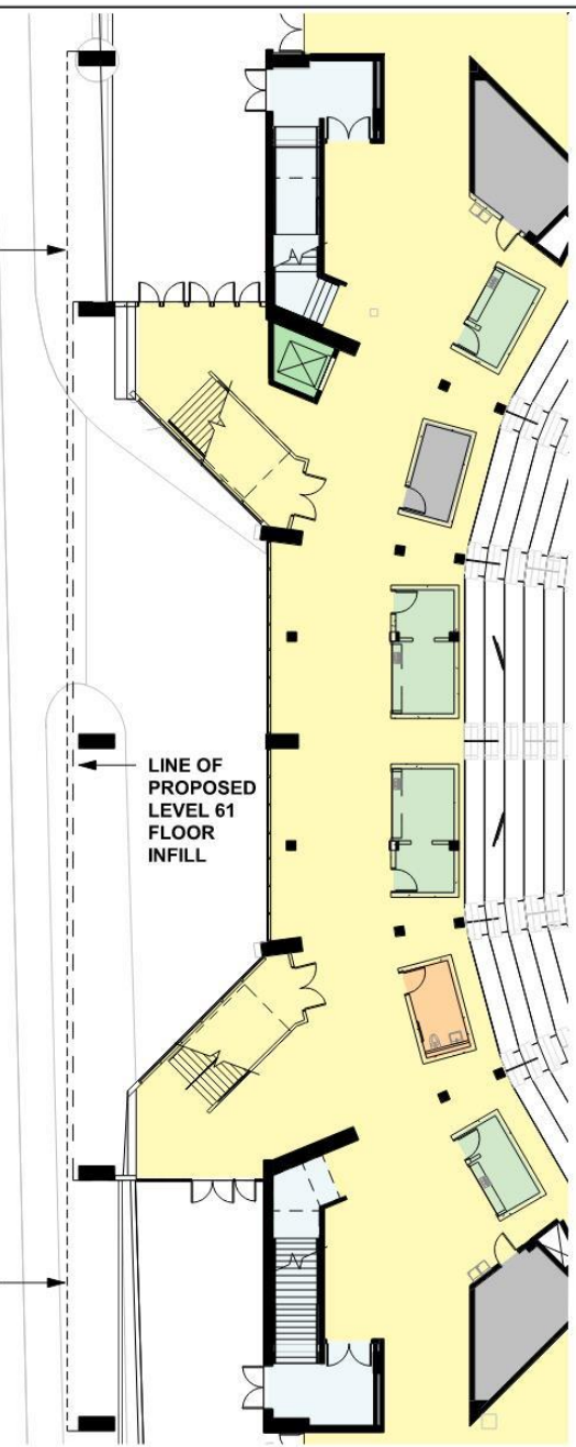
2 LEVEL 61 WEST - EXISTING FLOOR PLAN 1" = 20'-0"
